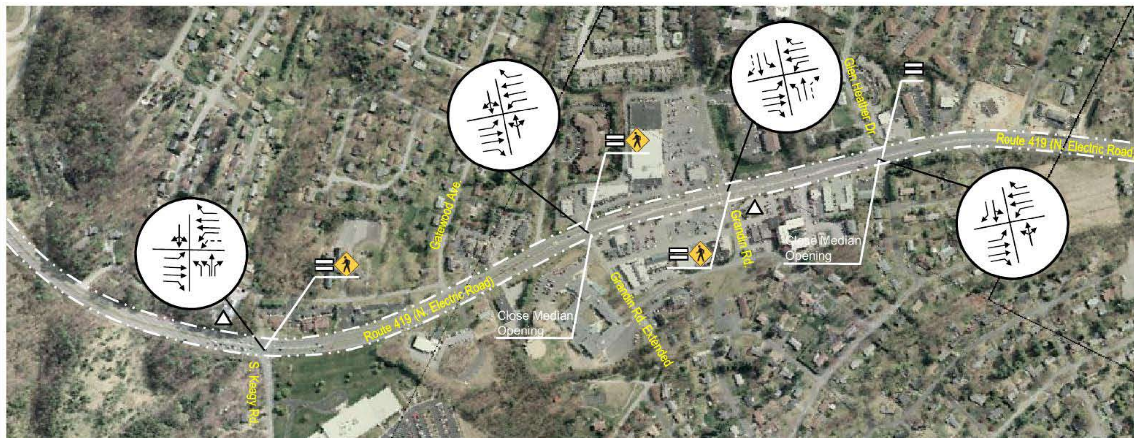
Figure 5.12 Recommended Improvements - Segment 6
