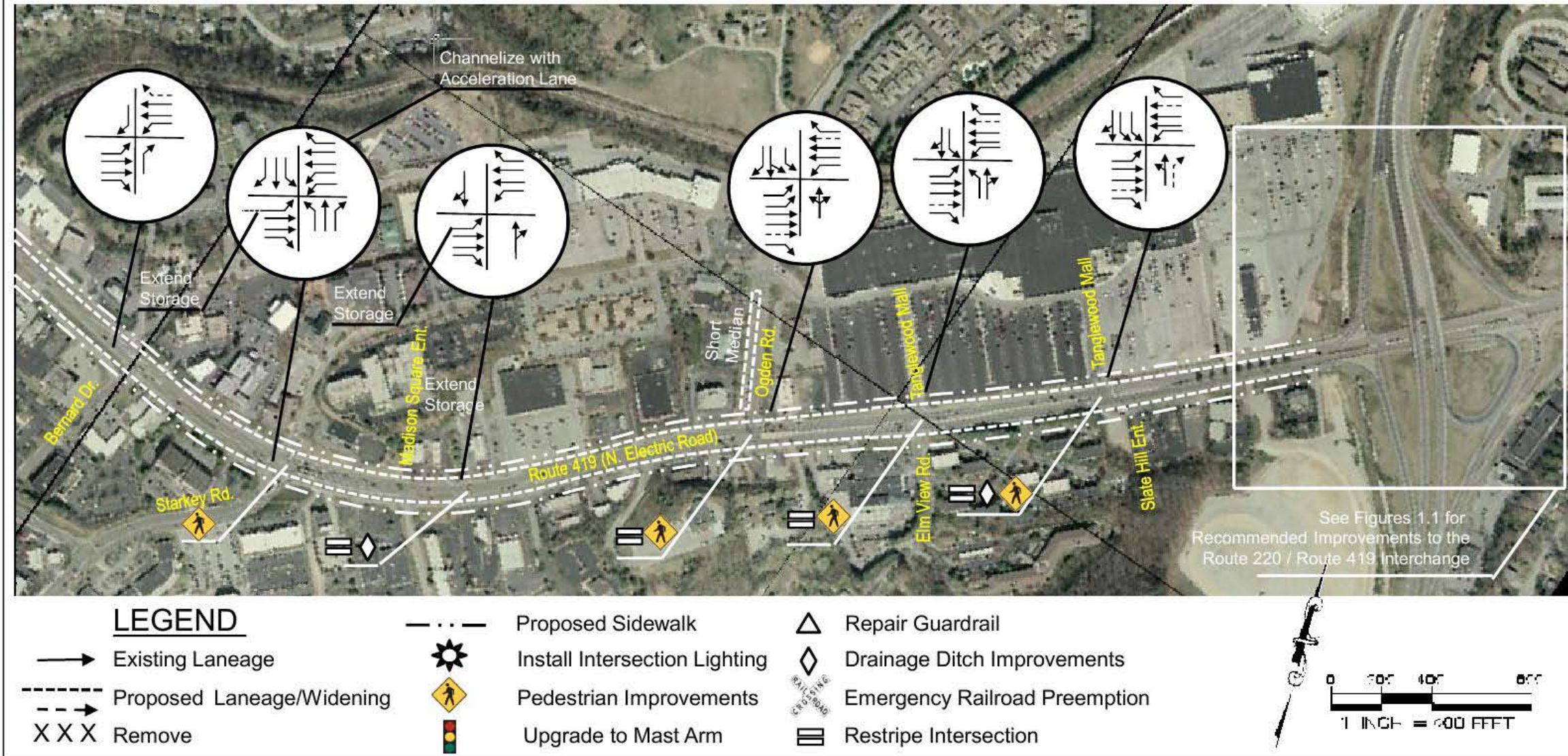
Figure 5.15 Recommended Improvements - Segment 9
