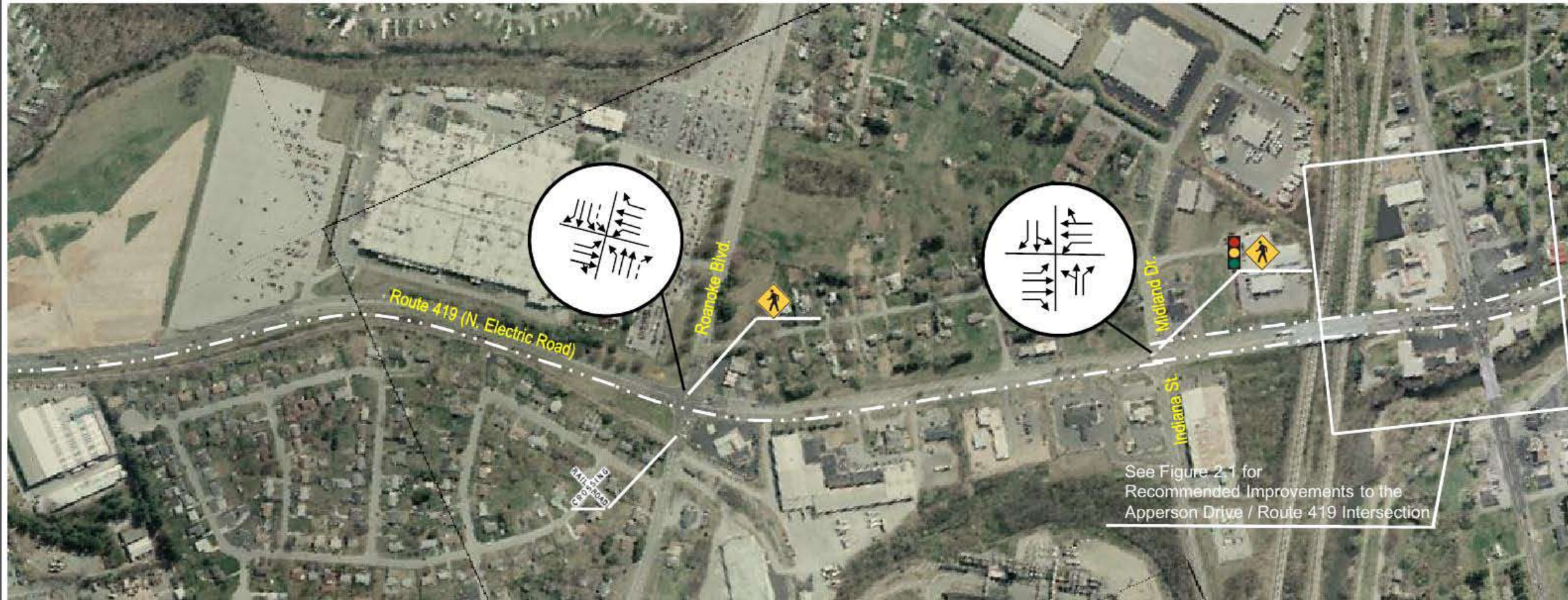
Figure 5.10 Recommended Improvements - Segment 4
