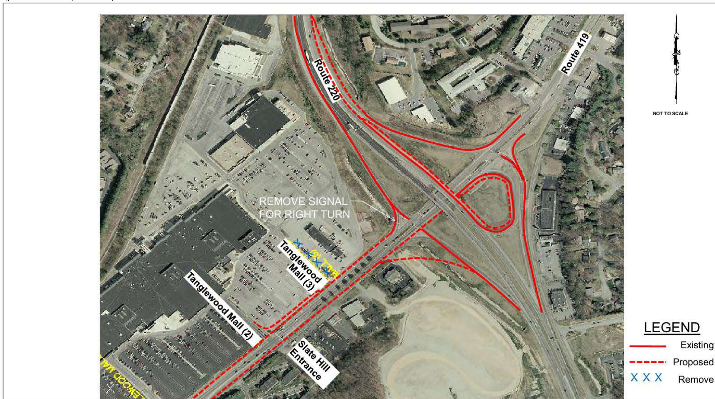
Figure 5.4 Route 419/US 220 – Option A
