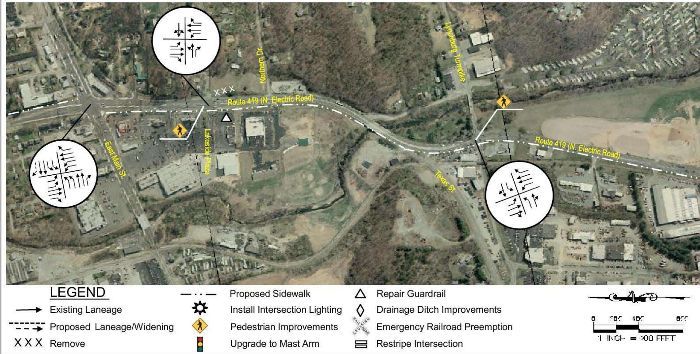
Figure 5.9 Recommended Improvements - Segment 3
