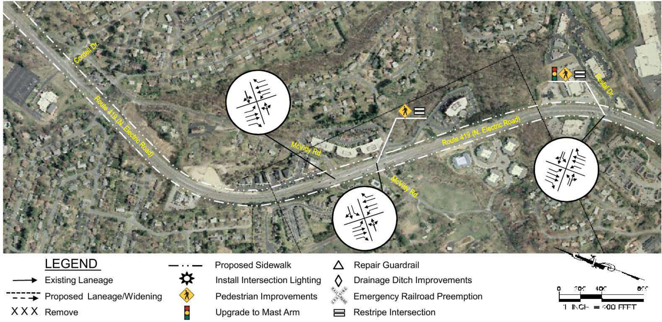
Figure 5.13 Recommended Improvements - Segment 7
