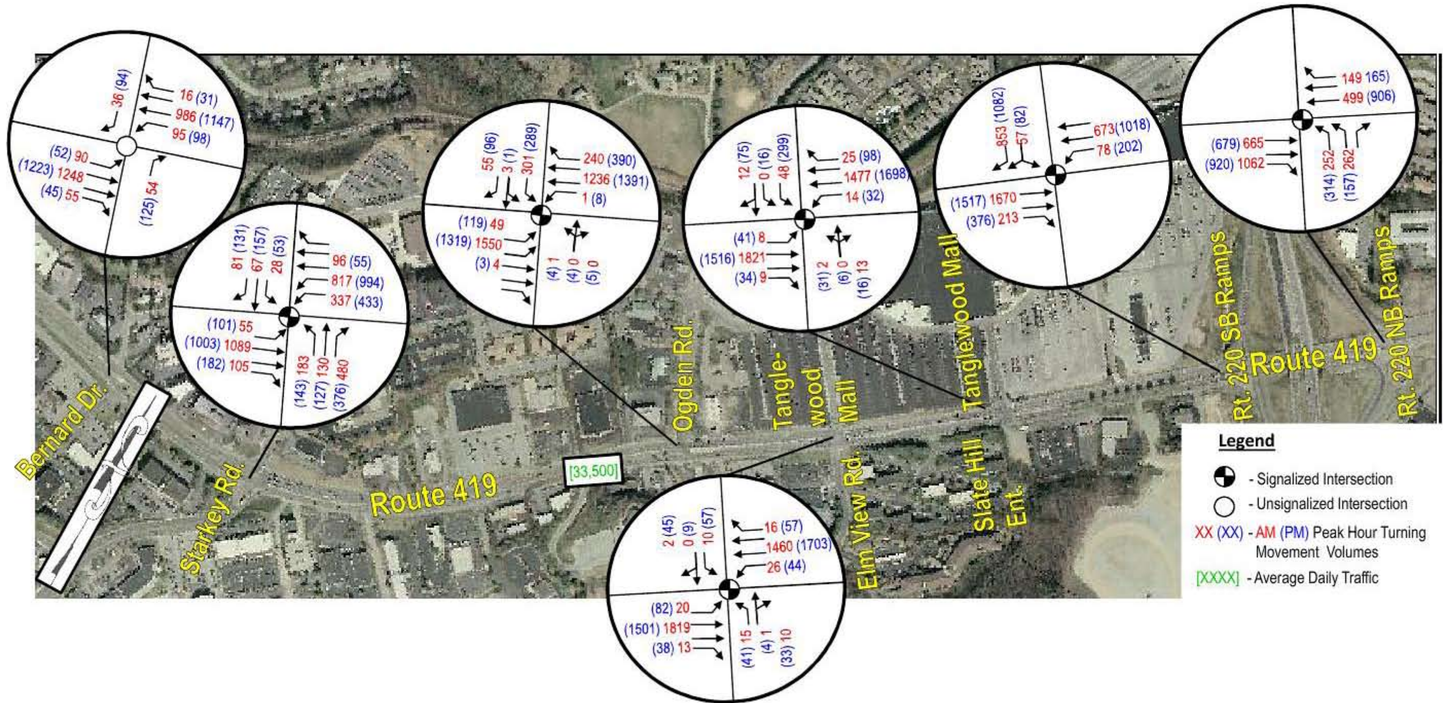
Figure 3.12 – Segment 9 (Bernard Drive to Franklin Road) Existing Geometry and Traffic Volumes
