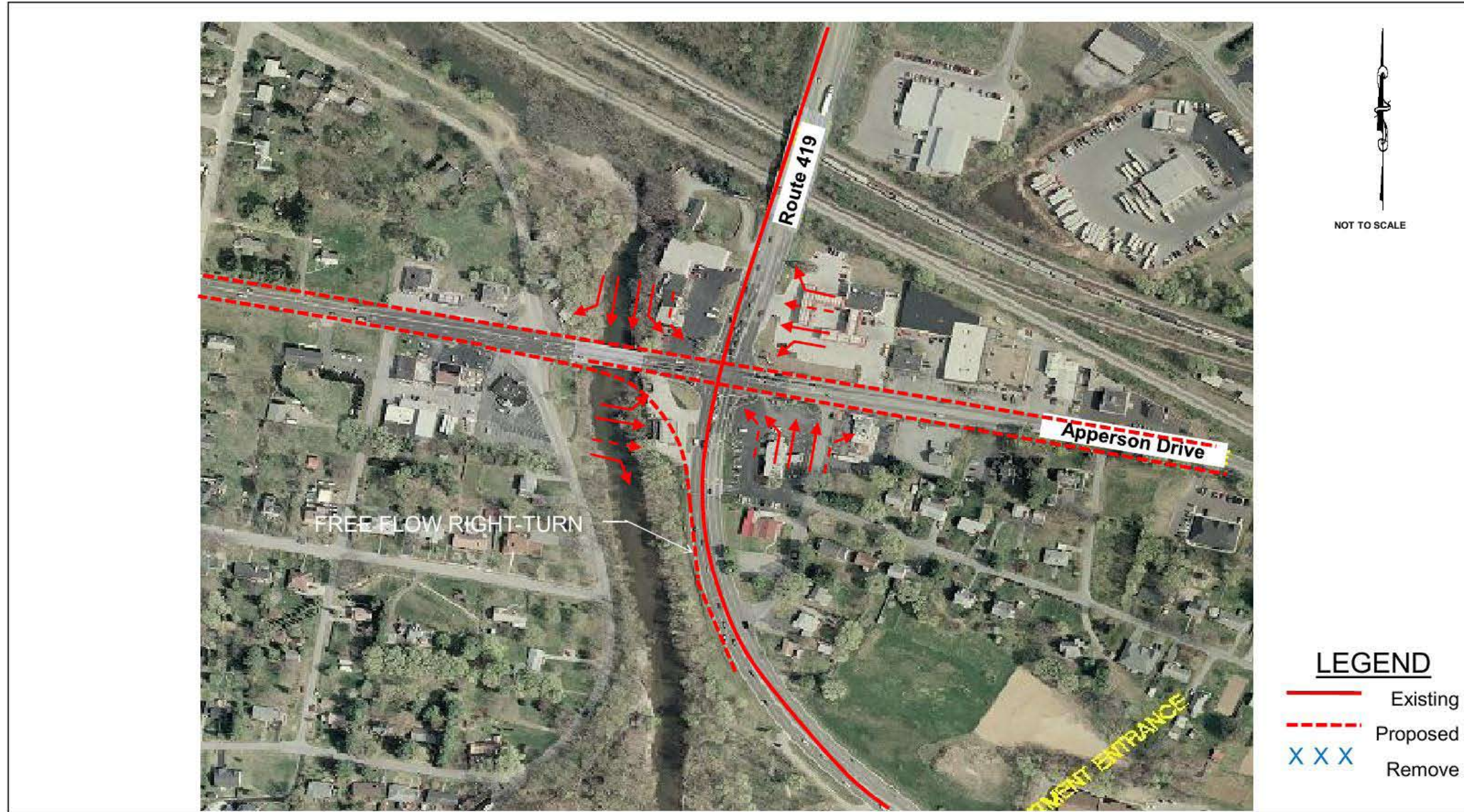
Figure 5.2 Route 419/Apperson Drive – Option A
