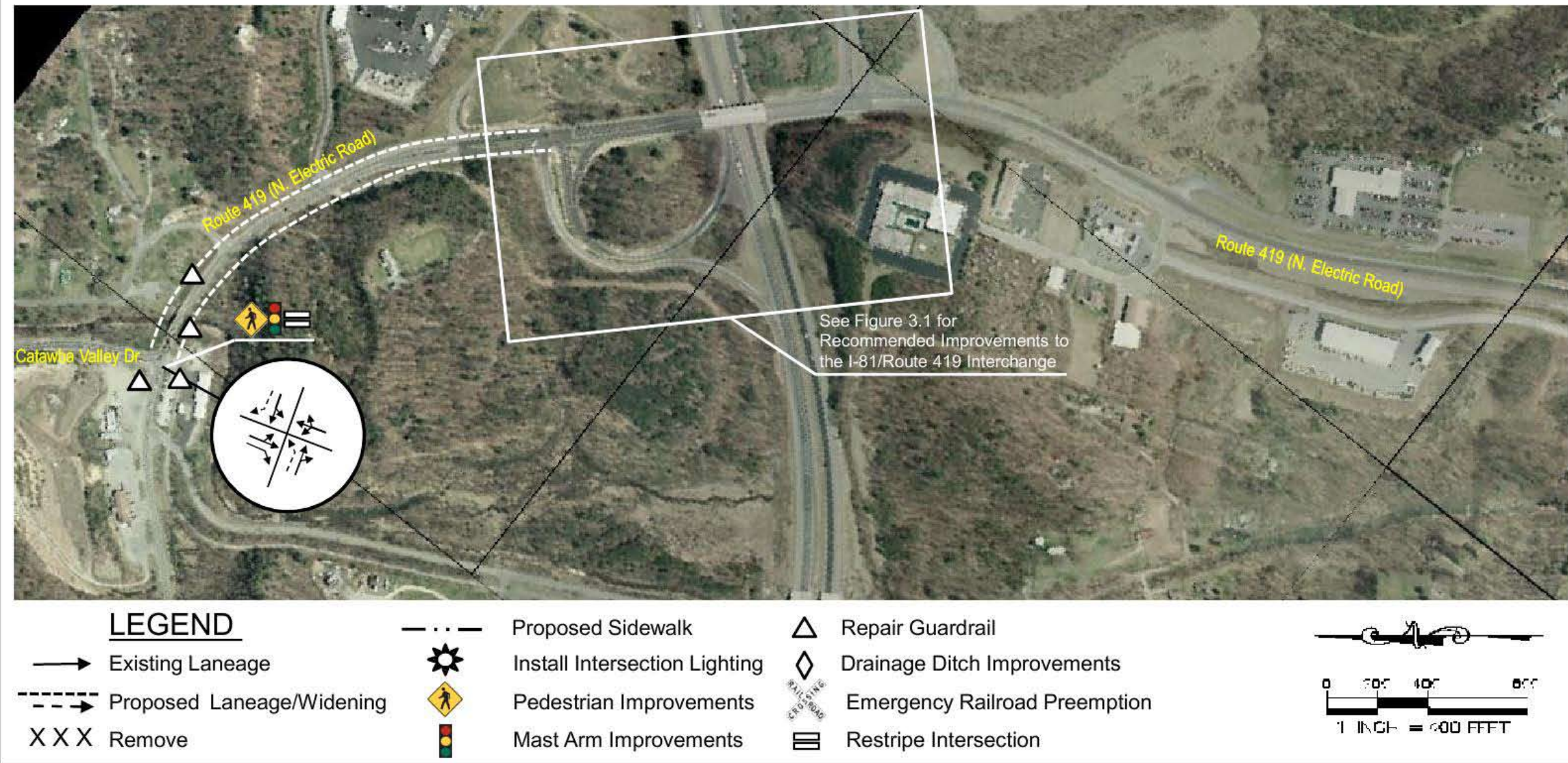
Figure 5.7 Recommended Improvements - Segment 1
