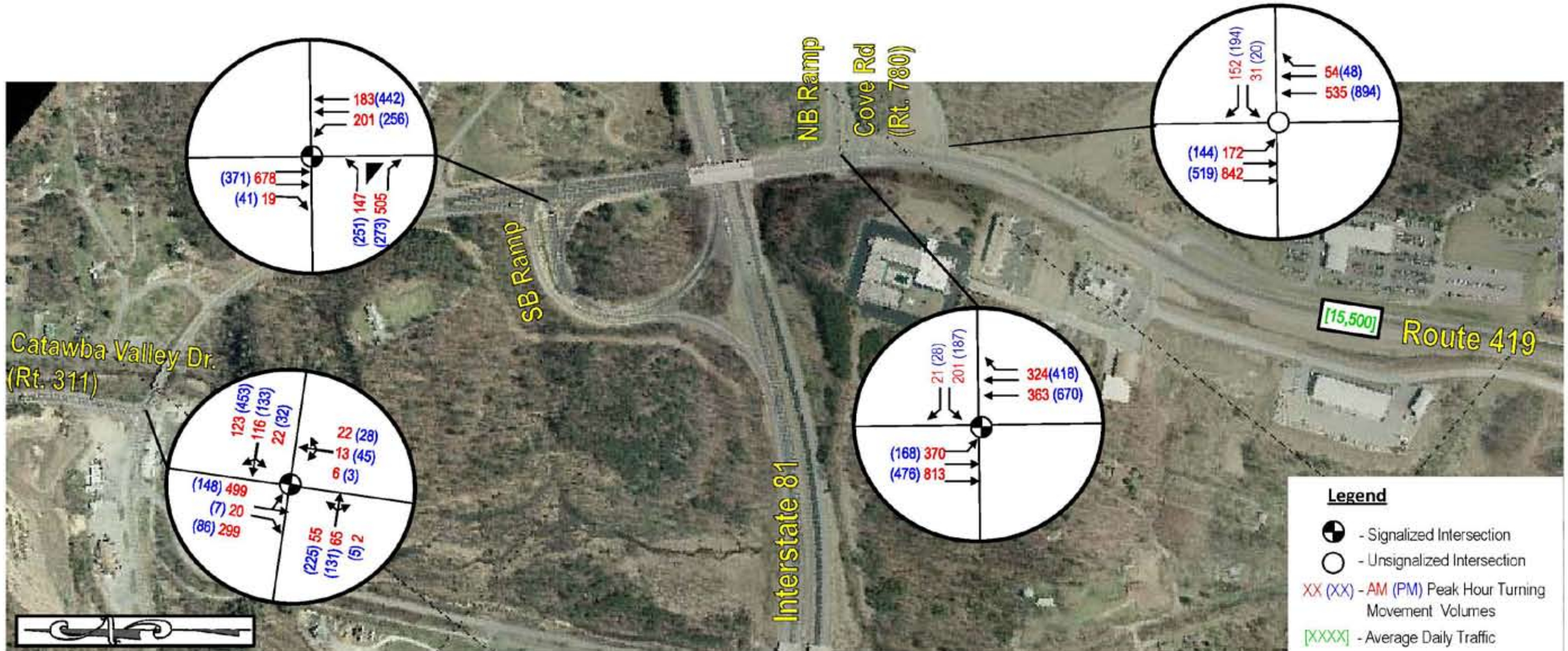
Figure 3.4 – Segment 1 (Kessler Mill Road to Sheraton Drive) Existing Geometry and Traffic Volumes
