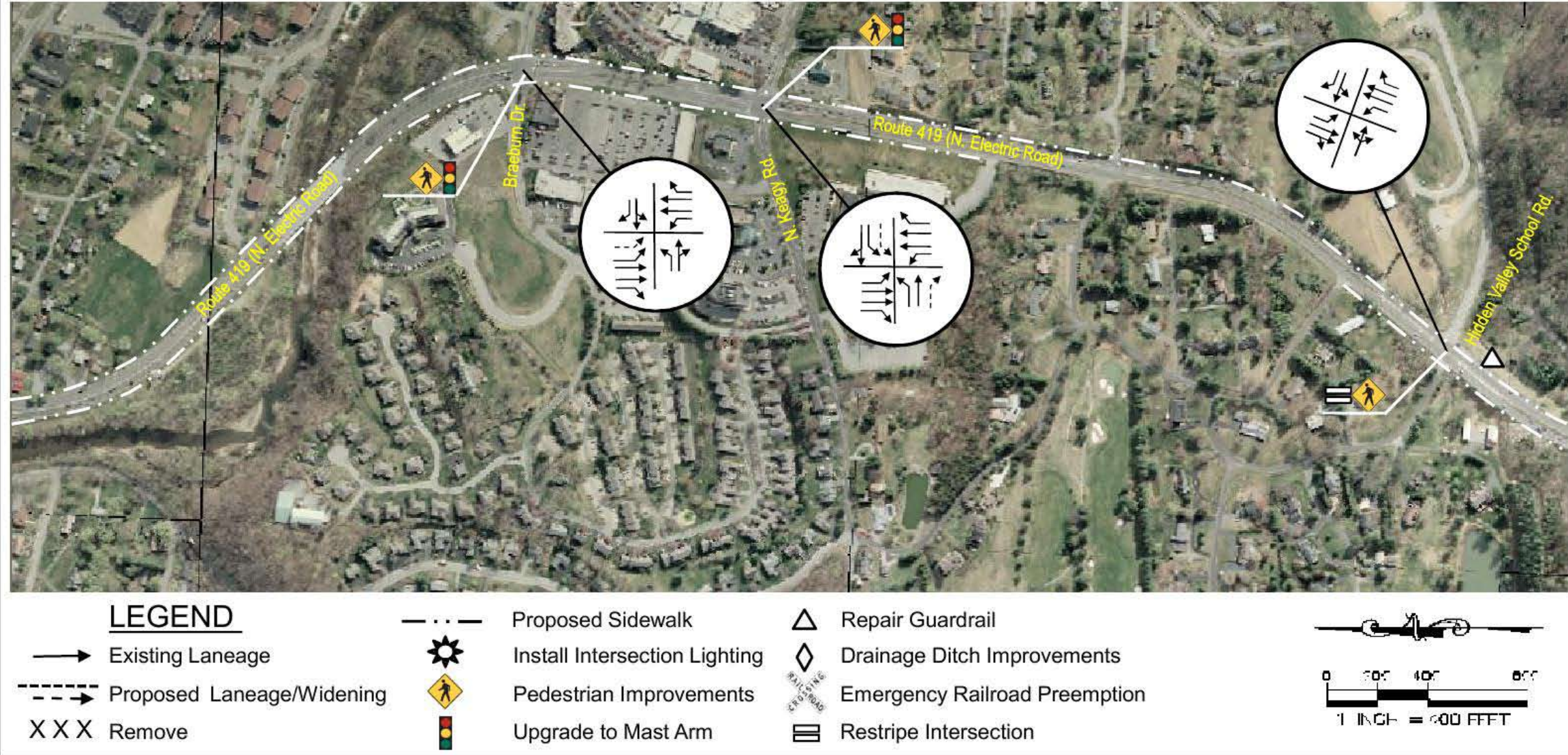
Figure 5.11 Recommended Improvements - Segment 5
