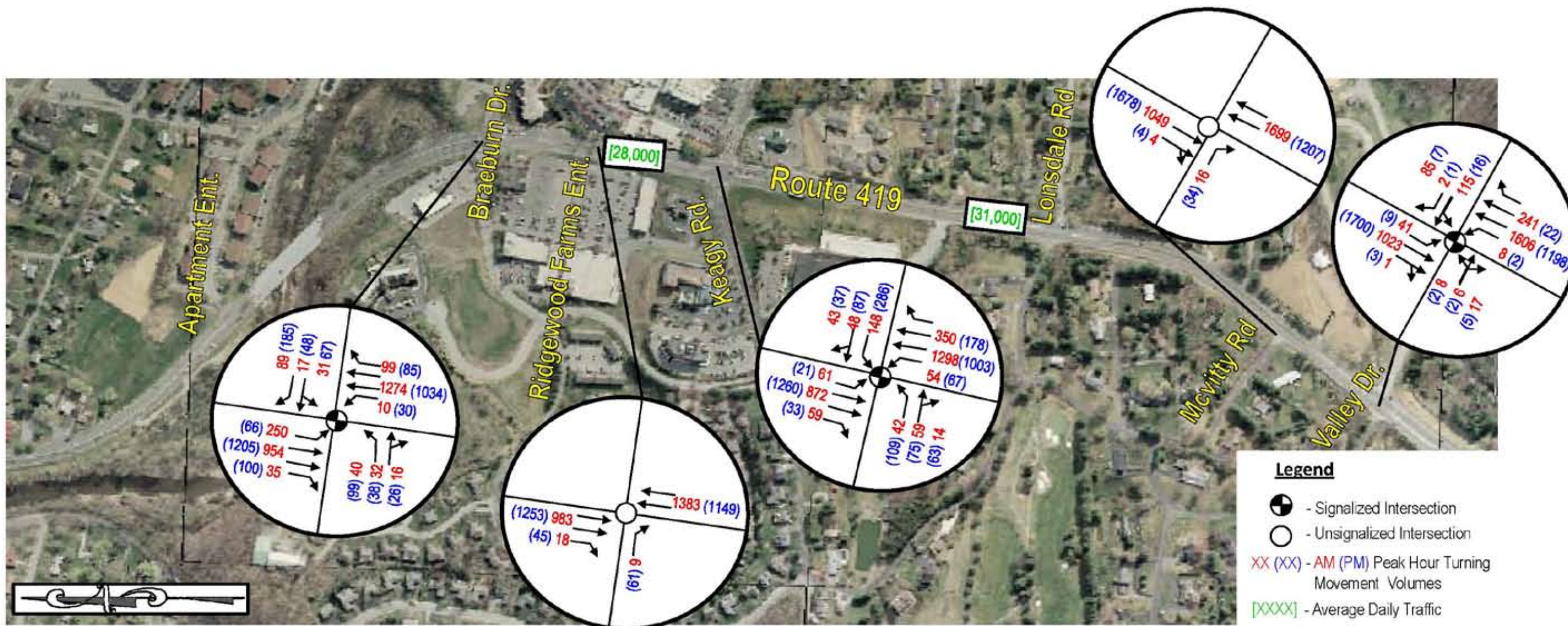
Figure 3.8 – Segment 5 (Riverview Drive to Dean Road) Existing Geometry and Traffic Volumes
