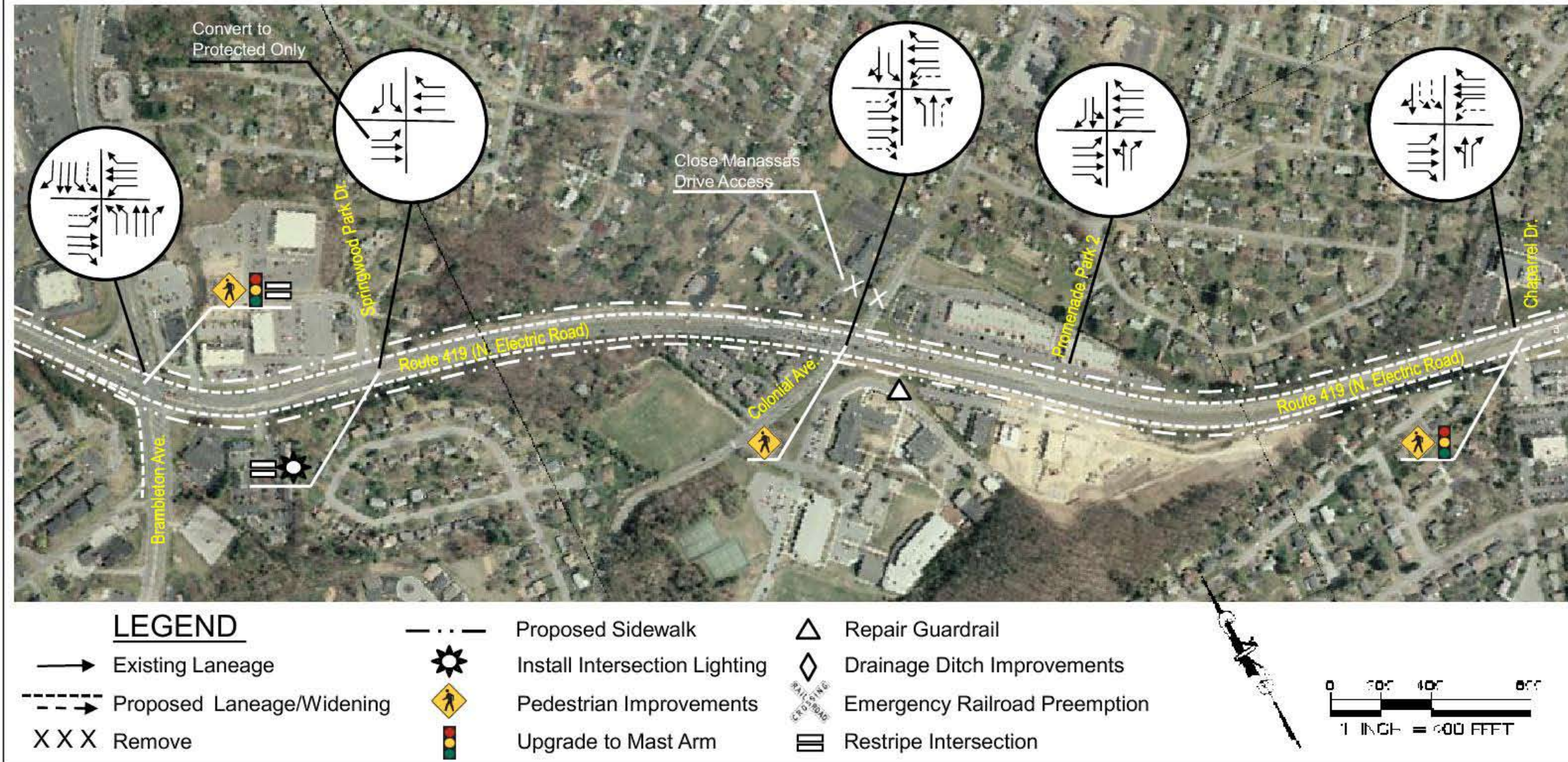
Figure 5.14 Recommended Improvements - Segment 8
