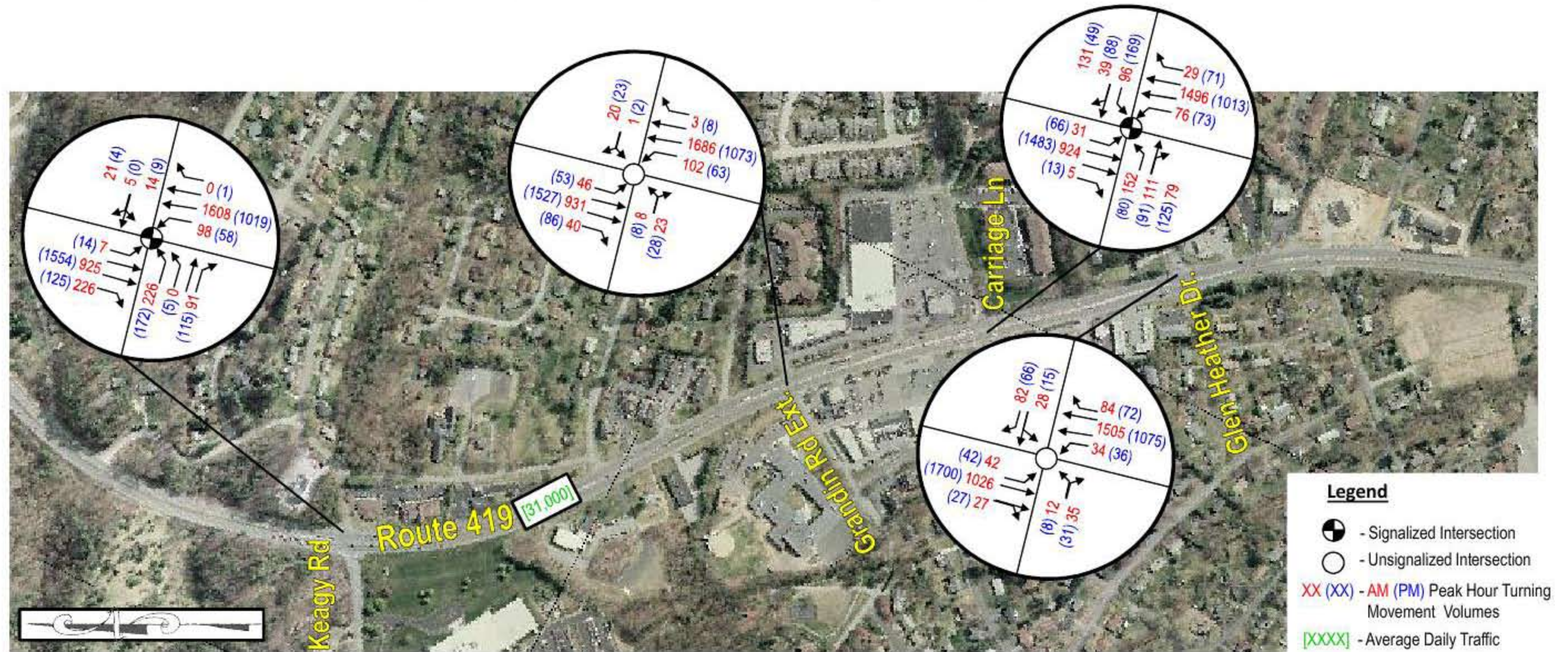
Figure 3.9 – Segment 6 (McVitty Road to Bower Road) Existing Geometry and Traffic Volumes
