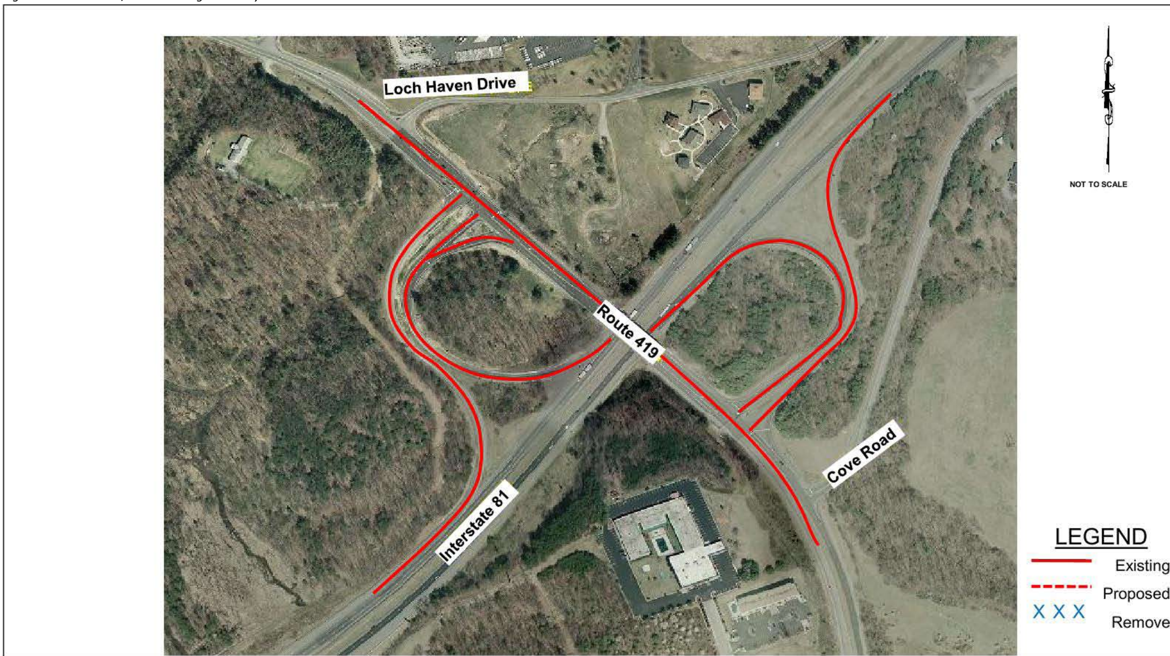
Figure 5.5 Route 419/I-81 – Existing Geometry
