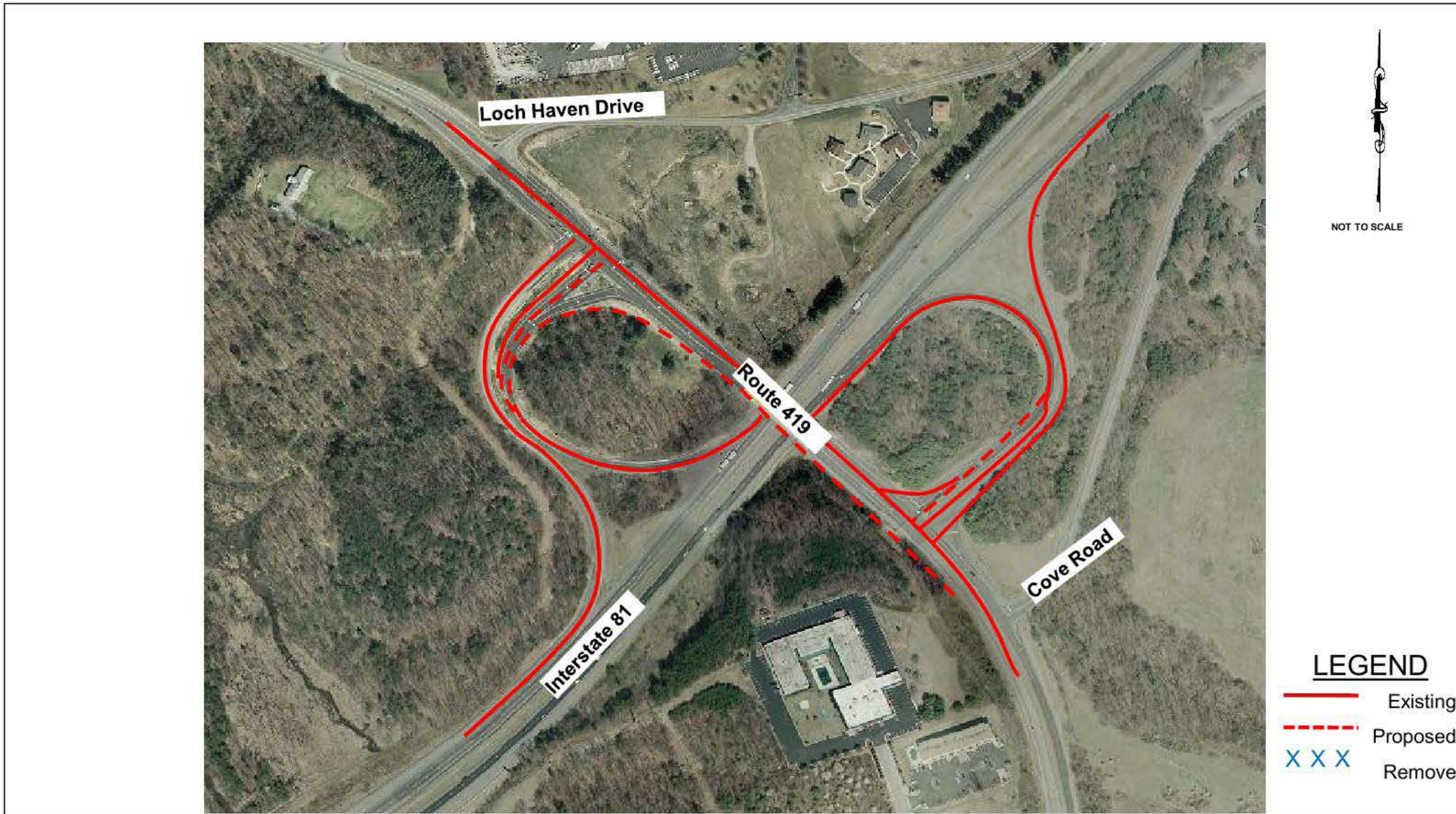
Figure 5.6 Route 419/I-81 – Option A
