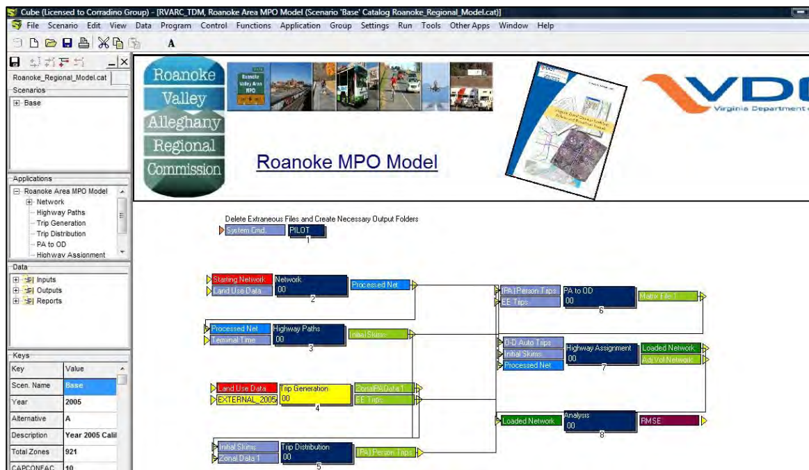
Figure 8- 5 RVTPO Model Catalog and Parent Application Snapshot
