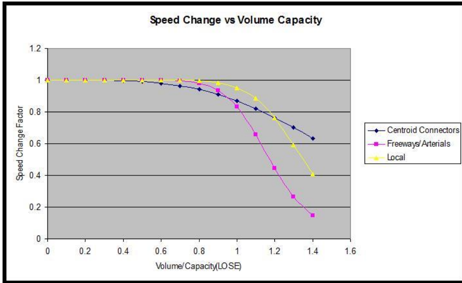
Figure 8- 4 Volume-Delay Curves - Base Year (2005) RVTPO Model
