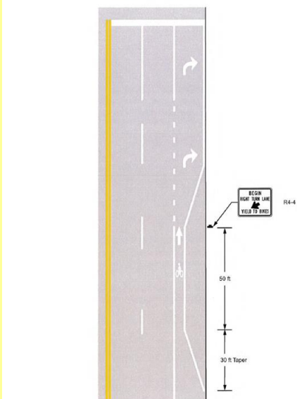
Figure 9C-4C. Example of Bicycle Lane Treatment at a Right-Turn Only Lane with Shoulder (Delaware Revision)
