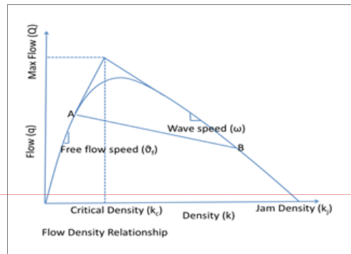
Figure 6-2 Flow Density Relationship
