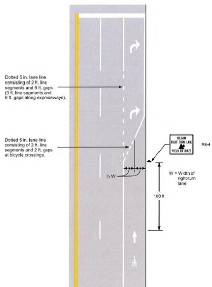
Figure 4- 15 Examples of Alternative Bike Accommodations
