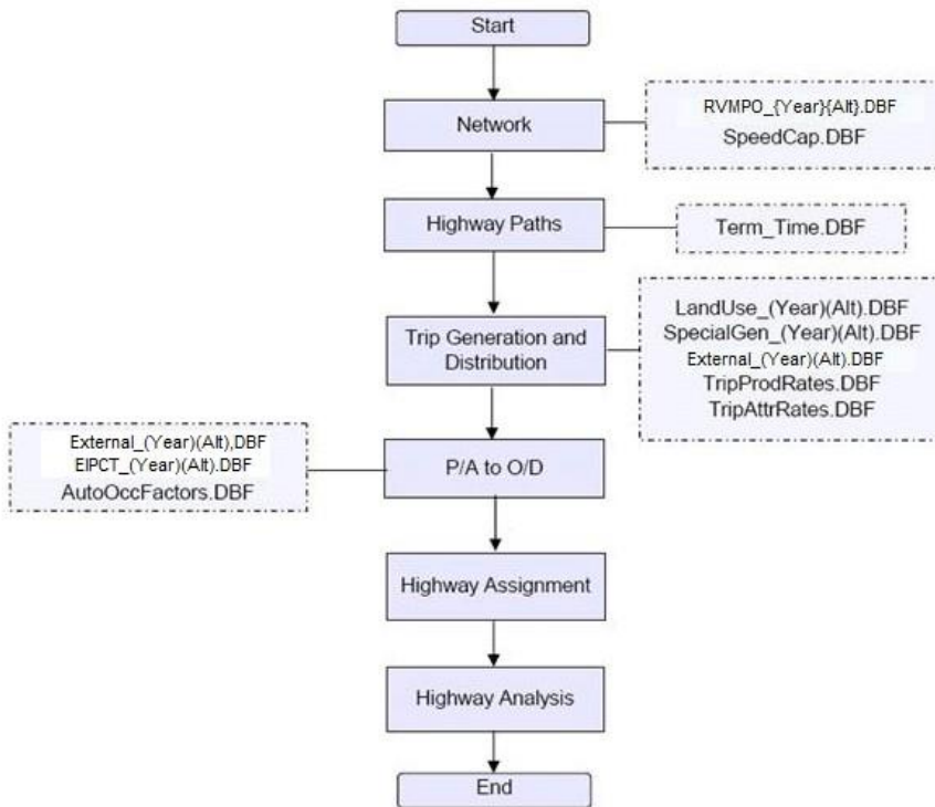
Figure 8- 1 Full Model Macro Flow Chart
